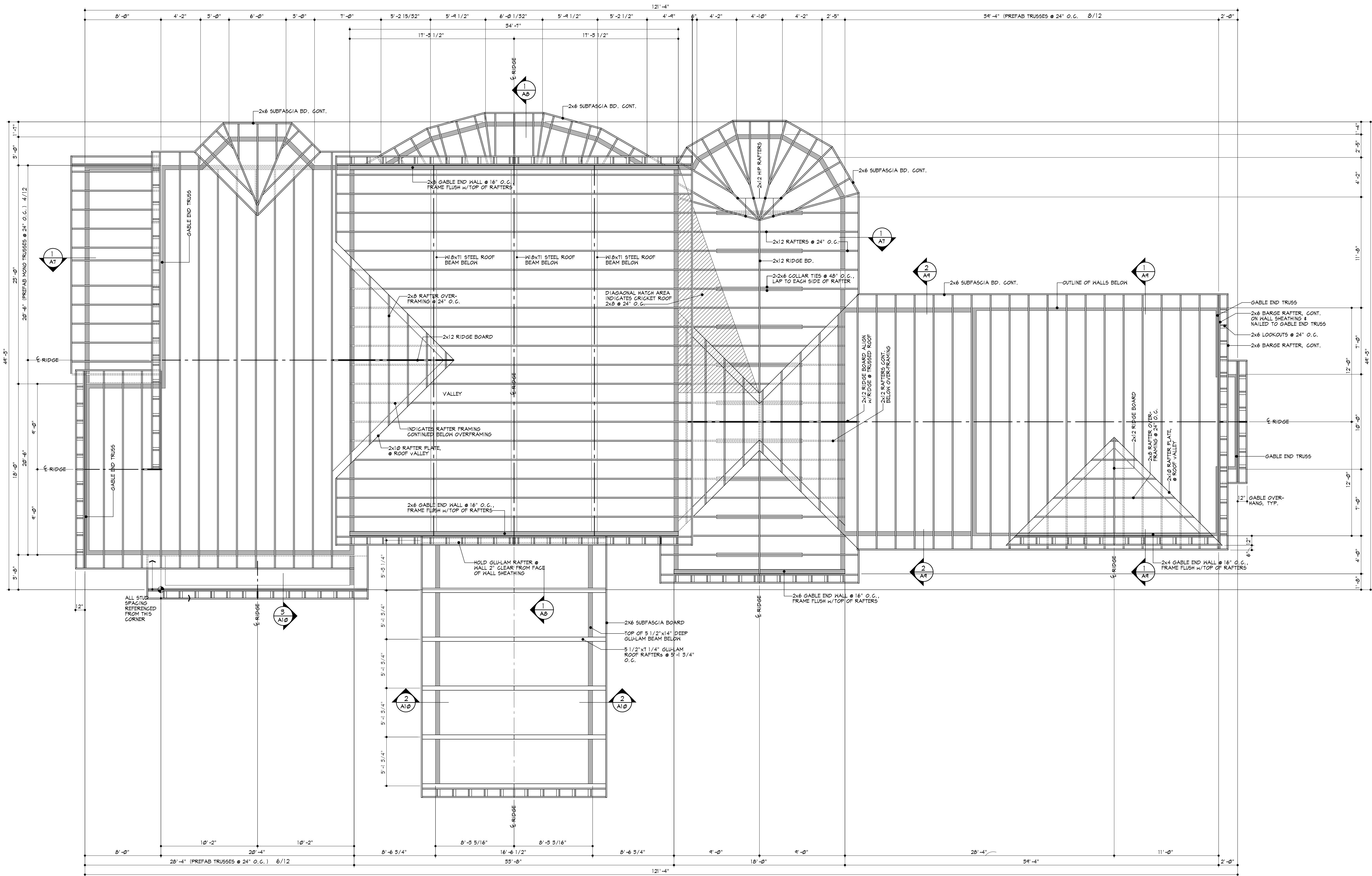
1 ROOF FRAMING PLAN A6 0 1 2 4 8'
